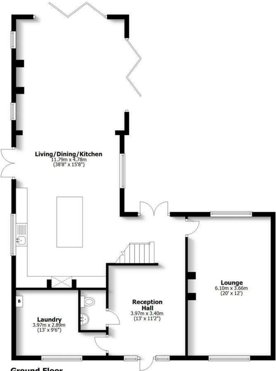
Ground Floor
